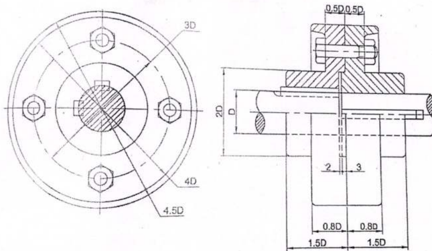
Fig. 8.3 Two Views of Protected Type Flange Coupling
